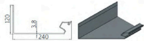
③ Rafter Profile
