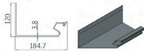
⑤ Side Gutter Profile
