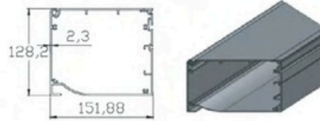
⑥ Motor Box Profile
