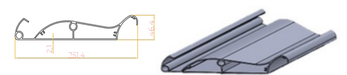
⑫ Panel Profili Aerofoil Louvre Profile
