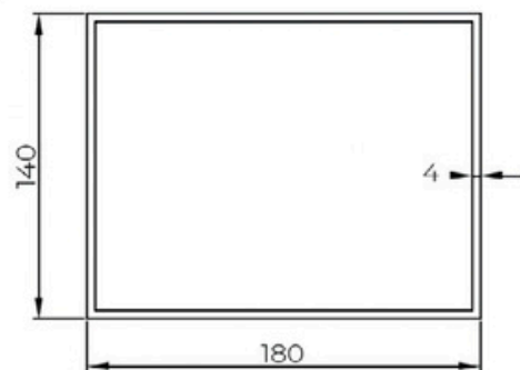
④ Profili Carrier Post Profile
