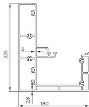
② Side Rafter & Gutter Profile
