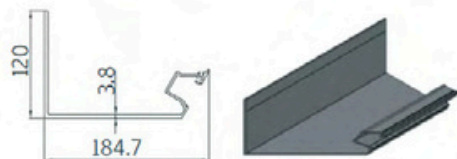
2 Side Gutter Profile
