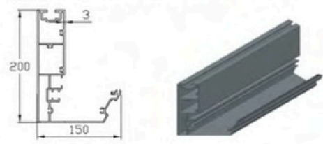
① Integrated Gutter & Rafter Profile
