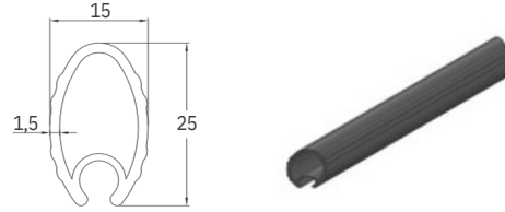
⑥ Valance Weight Bar
