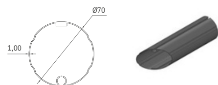
① Roller Tube \varnothing 70
