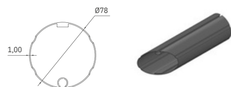
② Roller Tube \varnothing 78
