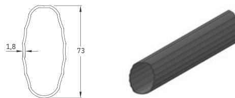
⑥ Arm Profile
