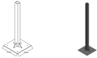
① Iron Post (Fixed To the Ground) 60x80
